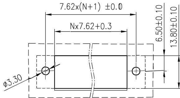
PANEL LAYOUT
