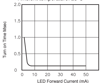
Fig.10 LED forward current vs. turn on time Across terminals 3 and 4 pin; Load voltage: 400V (DC); Continuous load current: 130mA (DC); Ambient temperature: 25°C
