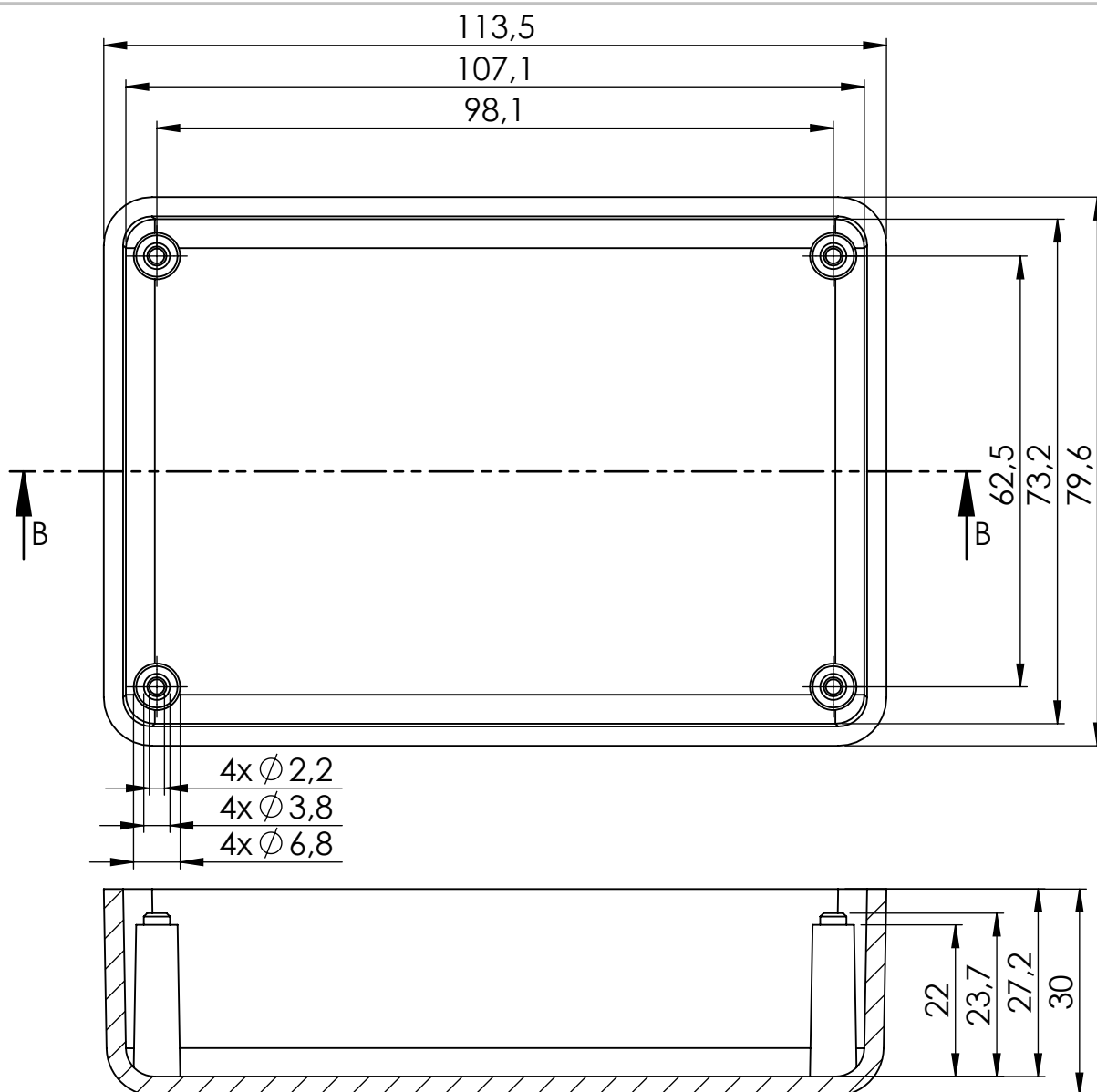
SECTION B-B
