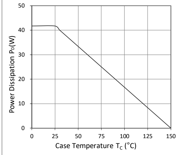
Figure 9. Power Dissipation
